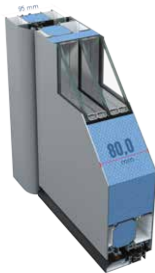
TLS90 CURVEDframe
