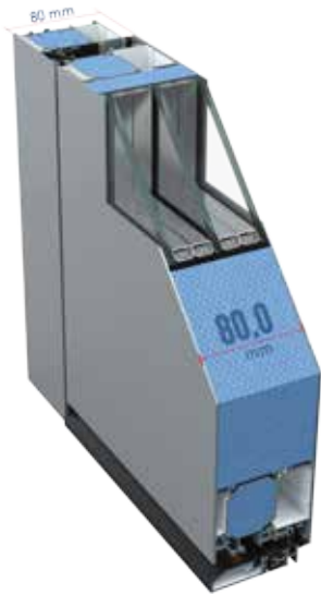
TLS90 FLATframe
