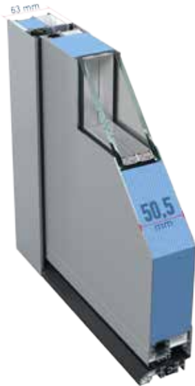
TLS50 FLATframe
