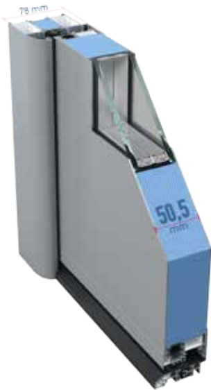
TLS50 CURVEDframe
